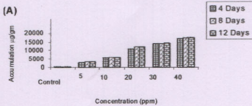
Fig: 3. Accumulation profile of Zinc by aquatic macrophytes (A) Salvinia (B) Spirodela
